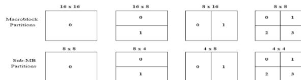
Figure 4. Macroblock partitions, sub-macroblock partitions and partition scans
