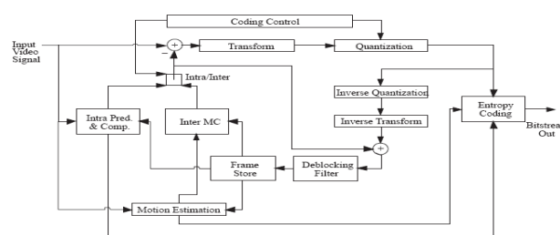
Figure 2. Basic coding structure of H.264/AVC for a MB
