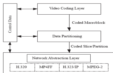
Figure 1. Structure of H.264/AVC video encoder
