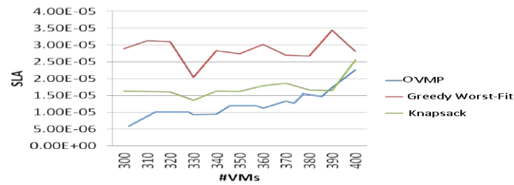
Figure 5: SLA
