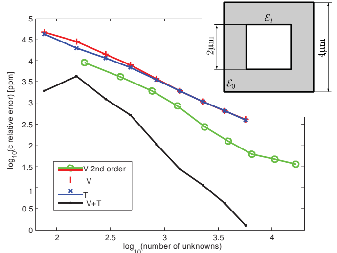
Fig. 6. Convergence of the p.u.l. capacitance value with respect to an increasing number of mesh elements for the square capacitor benchmark.
