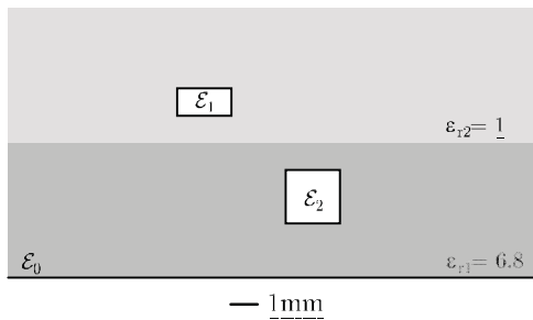
Fig. 7. MTL benchmark.
