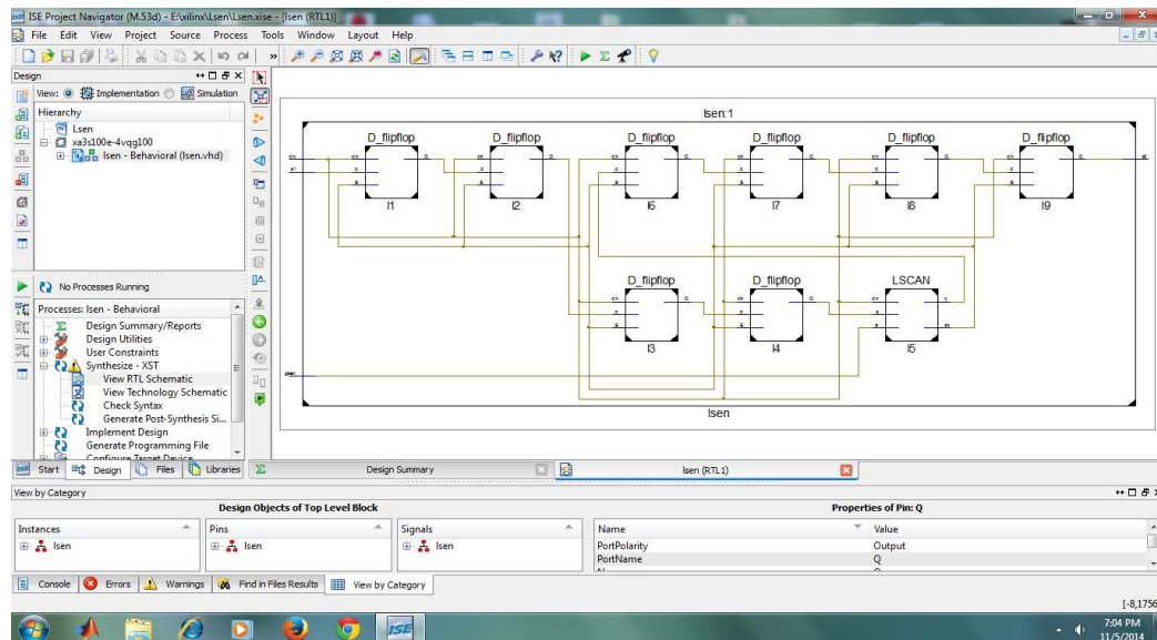
Figure 4.1 RTL schematic of LSEG cell
