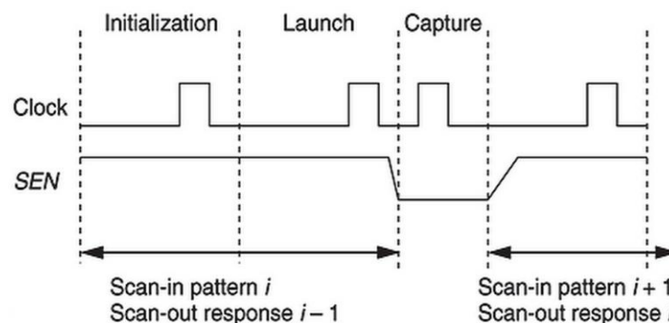
Figure 2.2 Waveform of Conventional LOC
