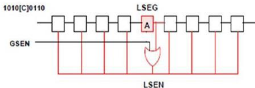
Figure 3.2 Local Scan Enable (LSEN) Generation
