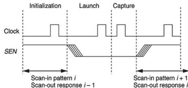
Figure 2.1 Waveform of LOS
