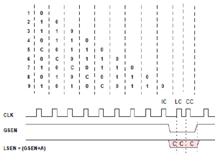
Figure 3.3 LSEN Generation Process
