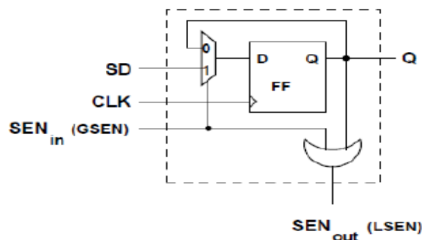
Figure 3.4 LSEG Cell
