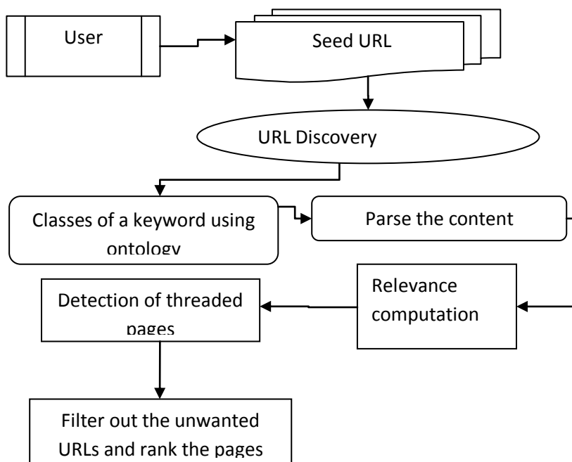
Figure 1: Multi keyword web crawling
